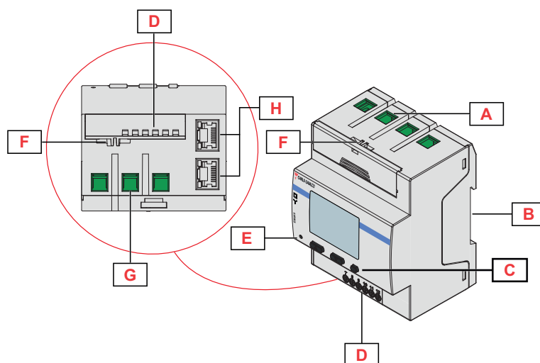
Fig. 1 EM640 front
